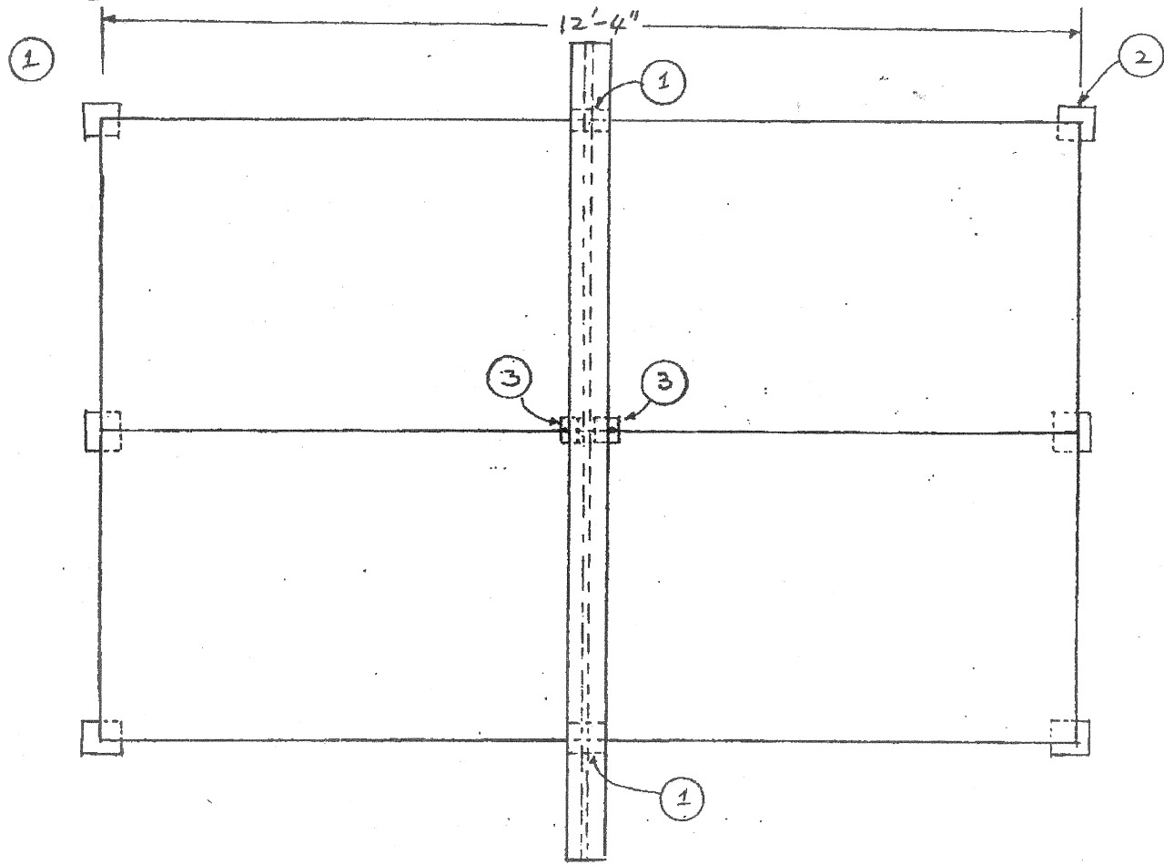
FIG. A-3: TEST SET-UP FOR CONNECTION SYSTEMS S1 TO S4
